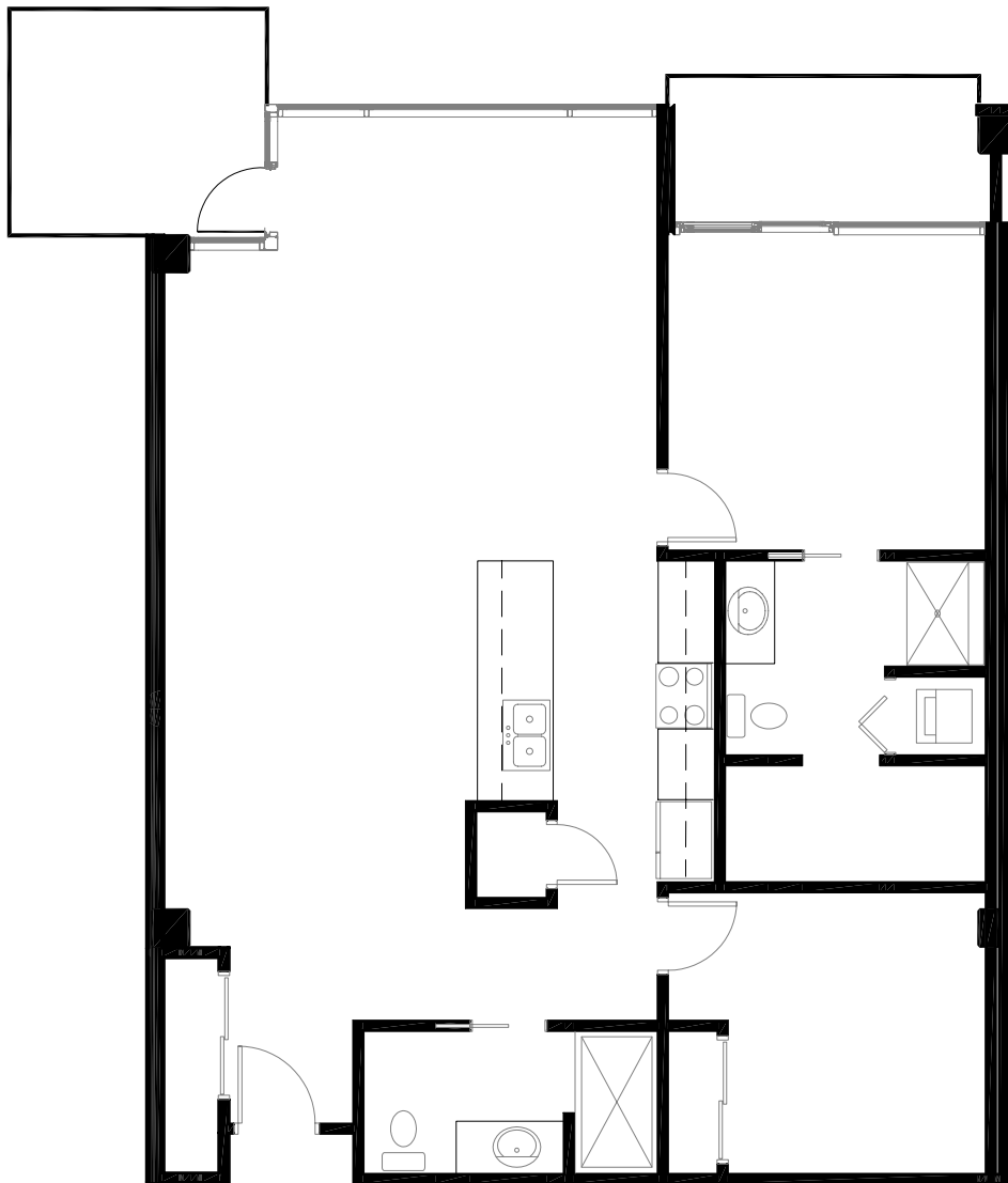
NW CORNER - UNIT 2 2ND FLOOR
