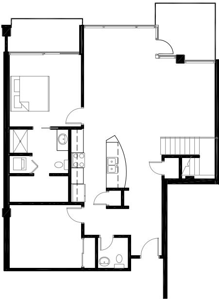
NE CORNER - UNIT 9 4TH FLOOR
